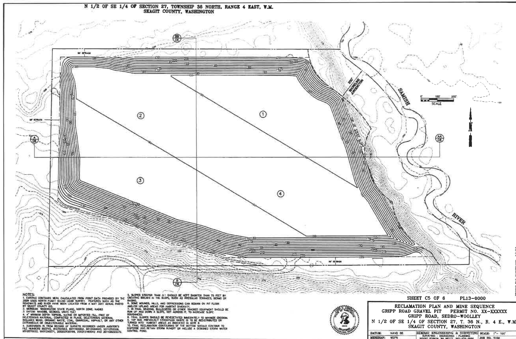
Figure 3. Proposed mining plan provided by Miles Sand and Gravel.
